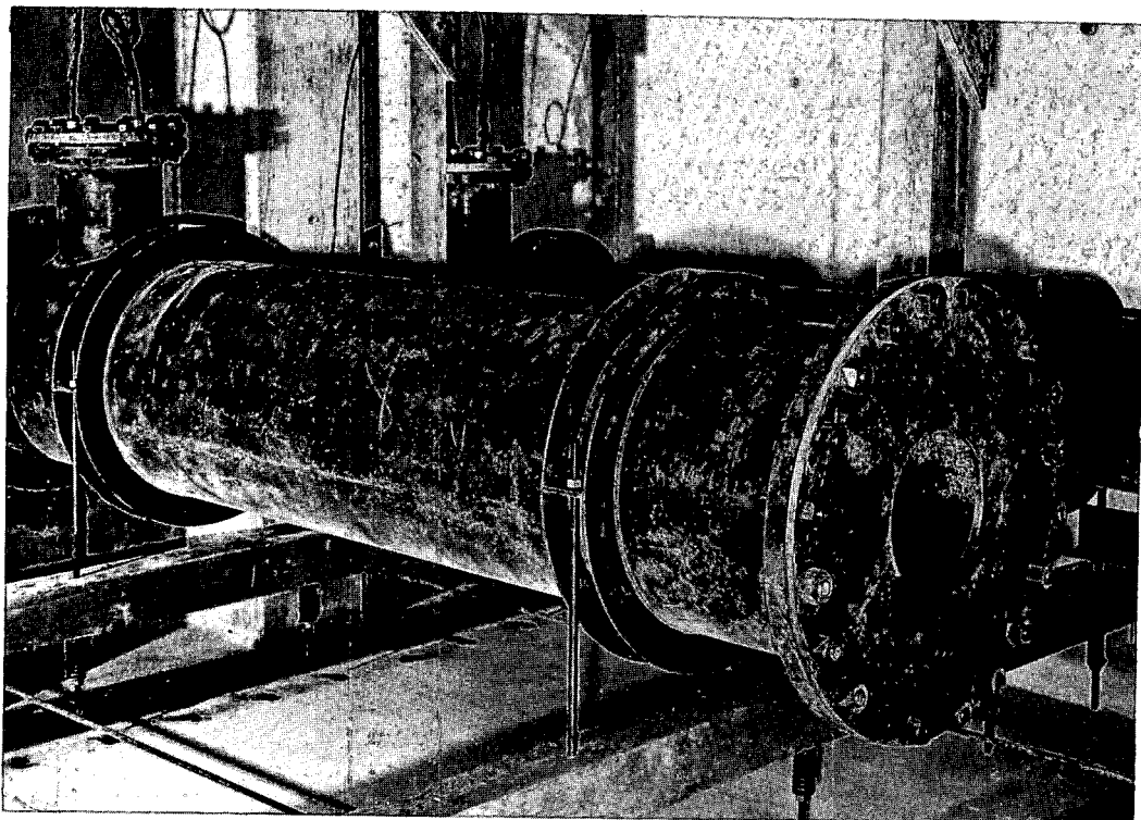
Fig. 6—Expansion chamber for horizontal valves at 7-psi range.
